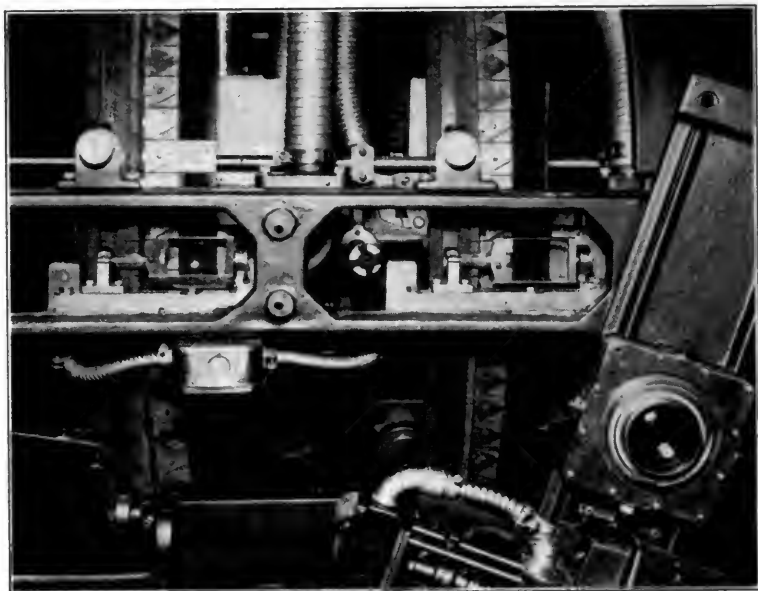
FIG. 2. Front with lens-plate removed, showing gear-teeth on slide-carriers and rotating plane-parallel plate for maintaining the picture stationary on the screen.
